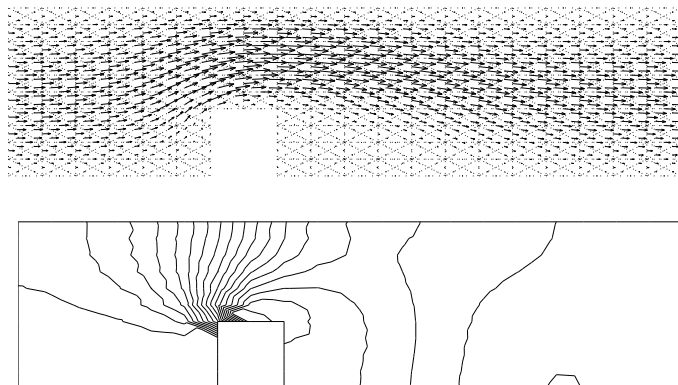
FIGURE 5. Approximate solution of the velocities and pressures at Reynolds number 100.
