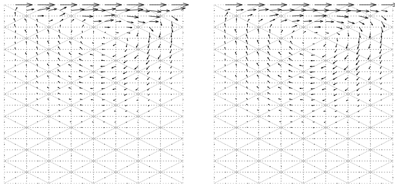
FIGURE 3. Approximate solution of the velocities, left: with fluxes only and right: with fluxes plus jump of the convective derivative.
