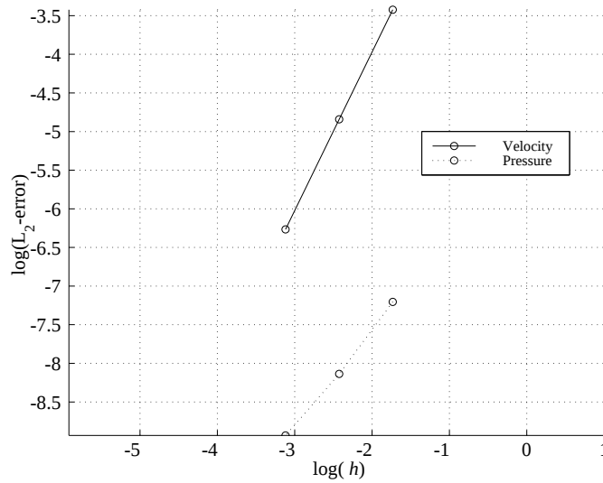
FIGURE 2. Convergence for \mu = 10^{-5}
