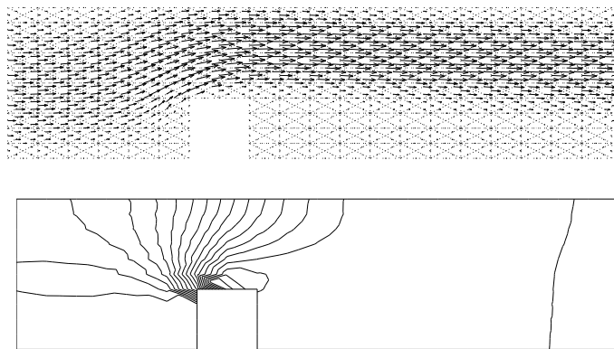
FIGURE 6. Approximate solution of the velocities and pressures at Reynolds number 1000.
