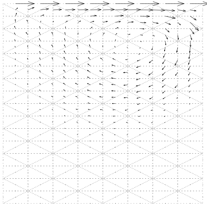
FIGURE 4. Approximate solution of the velocities with jump of the convective derivative only.
