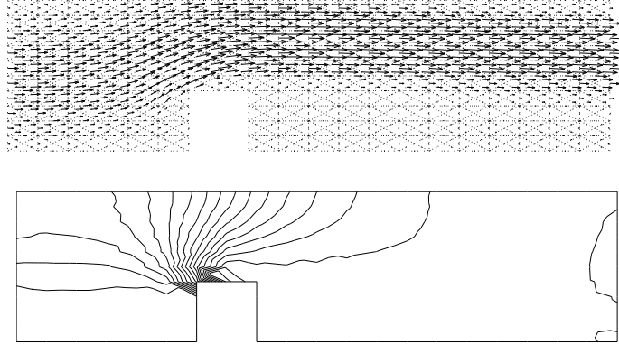
FIGURE 7. Approximate solution of the velocities and pressures at Reynolds number 10000.
