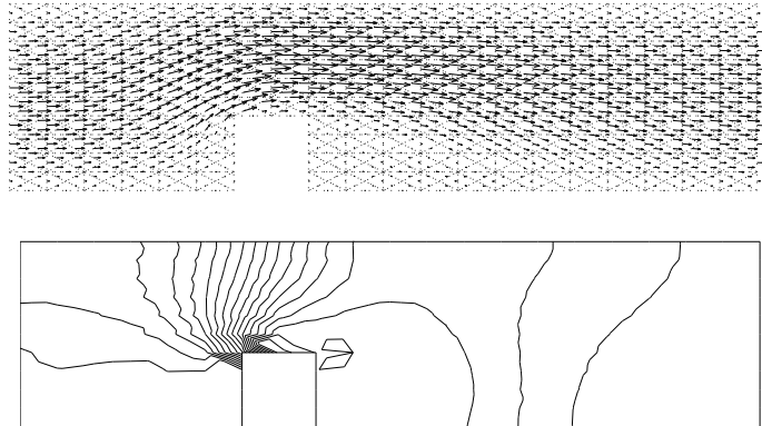
FIGURE 8. Approximate solution of the velocities and pressures at Reynolds number 10000, with fluxes.
