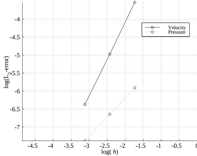
FIGURE 1. Convergence for \mu = 10^{-3}
